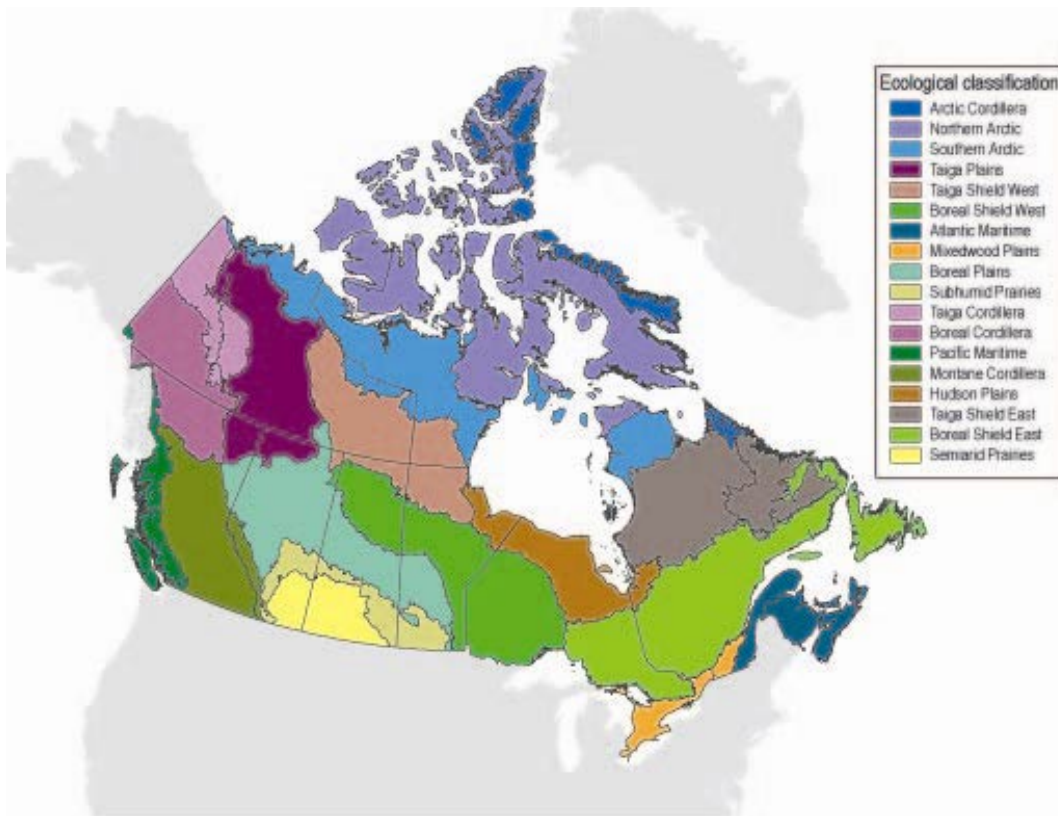
Figure A1: Terrestrial Ecozones of Canada (Environment Canada, 1996; Kull et al. , 2006).
