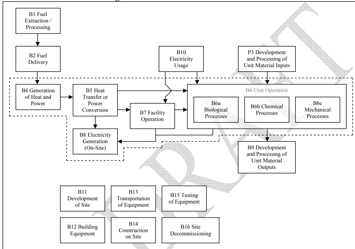
FIGURE 1.2: Process Flow Diagram for Baseline Condition
