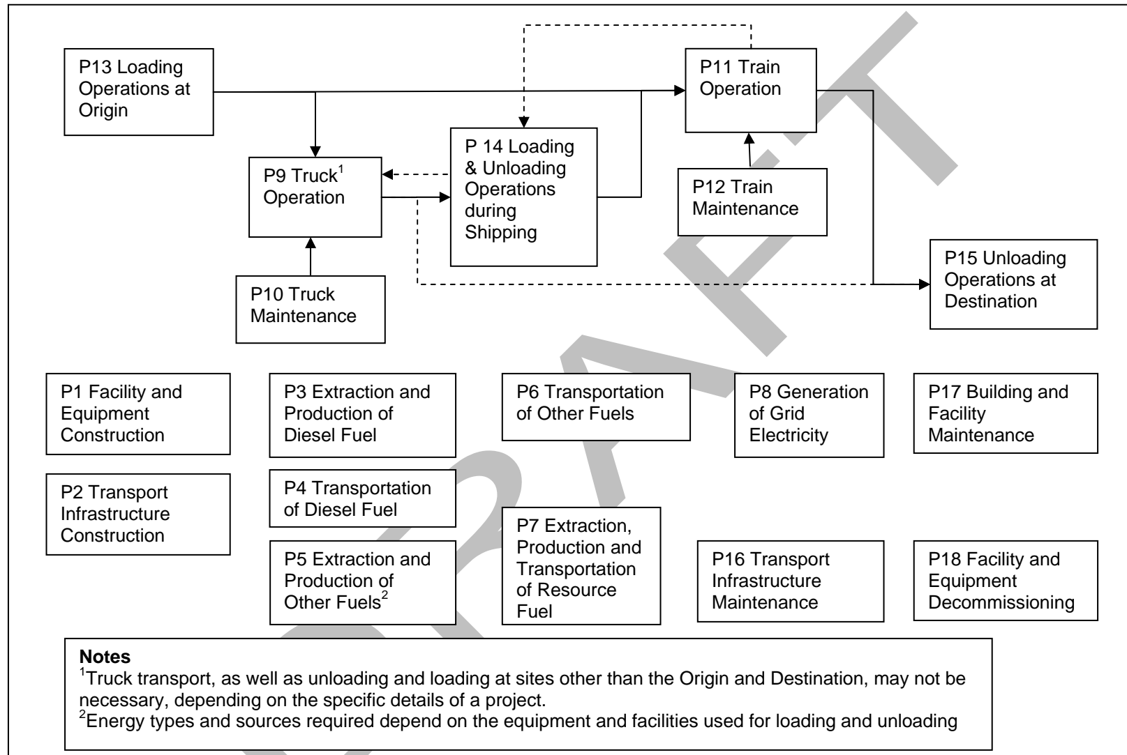
Figure 1-1: Process Flow Diagram for Project Condition
