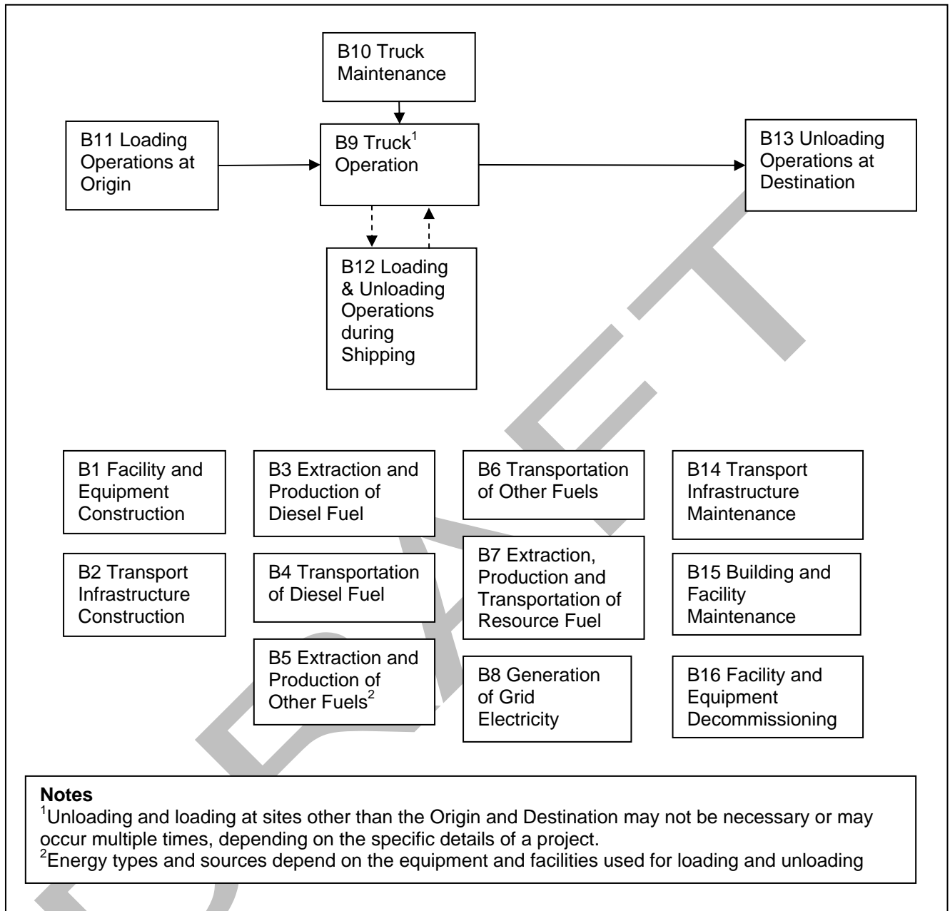
Figure 1-2: Process Flow Diagram for Baseline Condition
