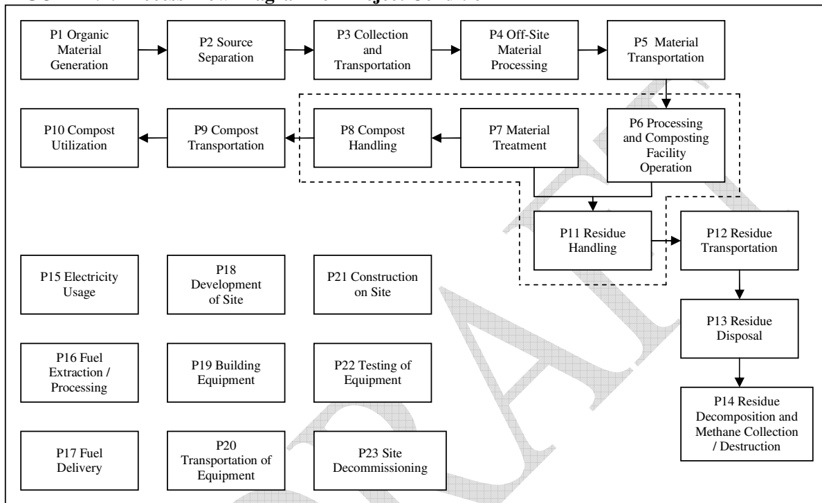
1 FIGURE 1.1: Process Flow Diagram for Project Condition
